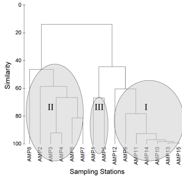
Fig 2. Amphipods in Probolinggo and Tangerang as determined by cluster analysis based on Bray–Curtis similarity coefficient
